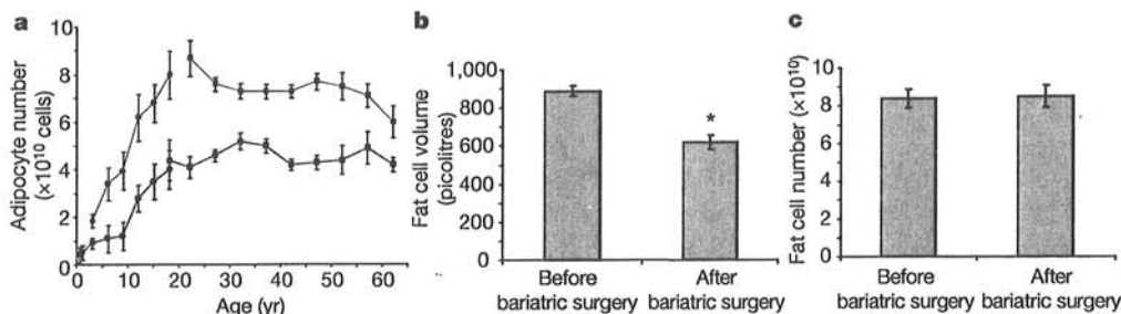
Figure 2 | Adipocyte number remains stable in adulthood, although significant weight loss can result in a decrease in adipocyte volume. Total adipocyte number from 595 ( n lean = 253; n obese = 342) adult individuals (squares) was combined with previous results for children and adolescents 8 (circles; n lean = 178; n obese = 120). a, The adipocyte number increases in
